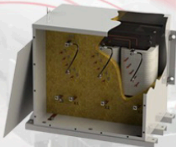
Step-Up / Step-down Power Transformer
